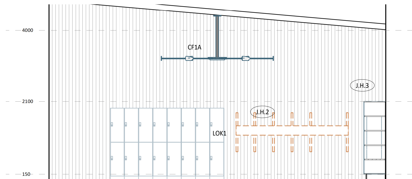
4 ELEVATION DETAIL 60-003 1 : 50
