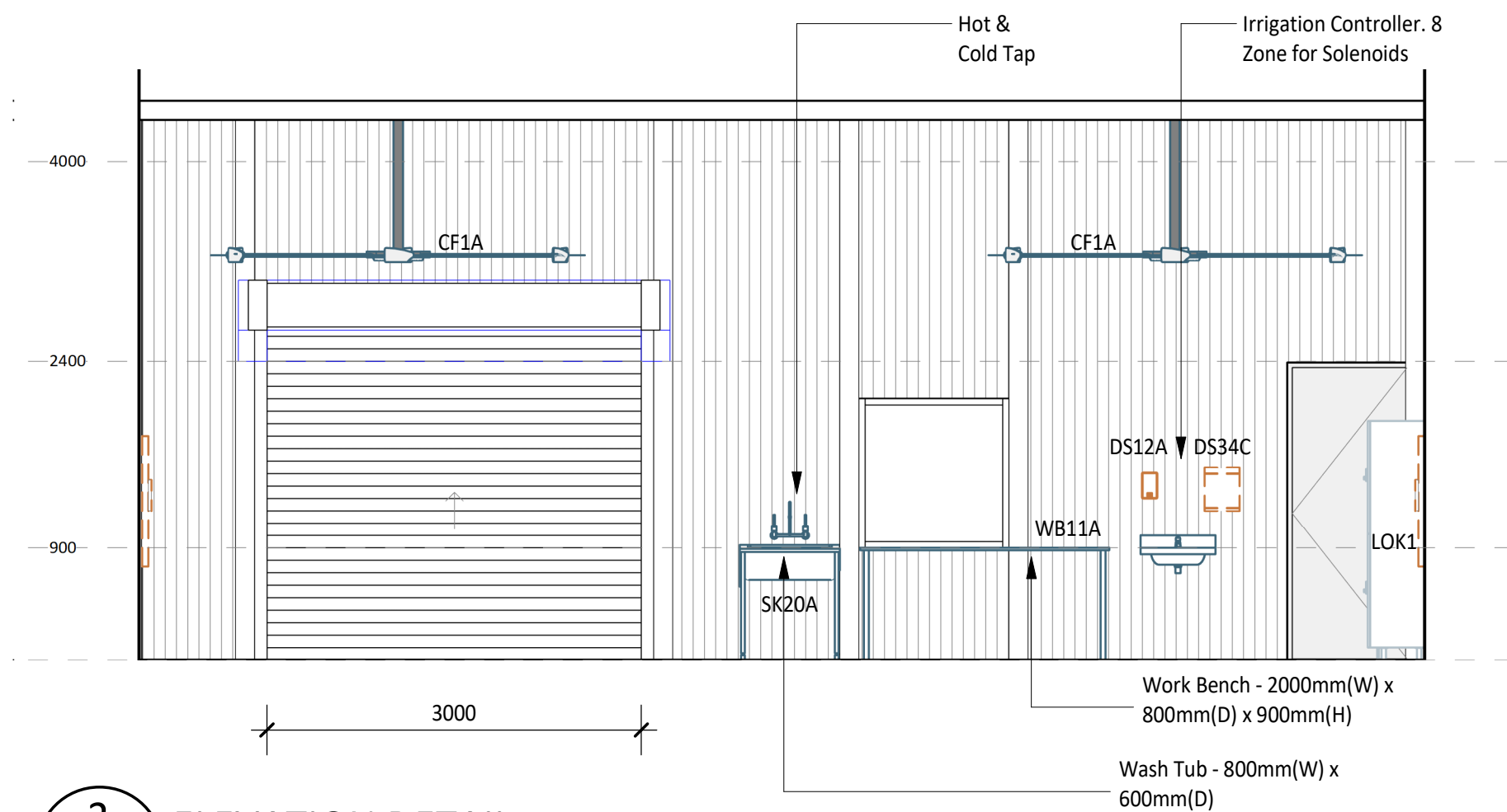
3 ELEVATION DETAIL 60-003 1 : 50
