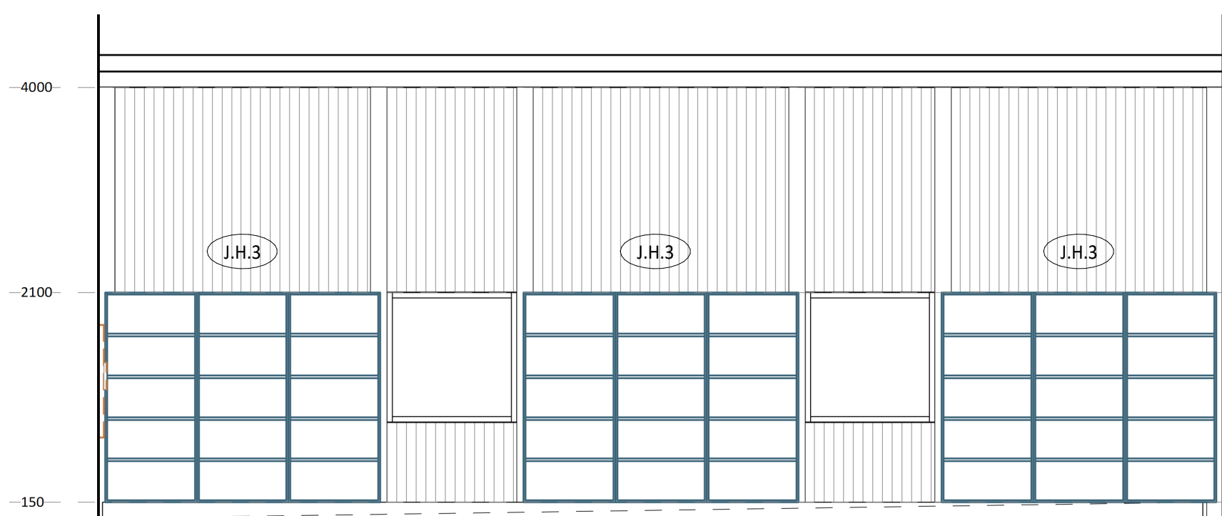
5 ELEVATION DETAIL 60-003 1 : 50
