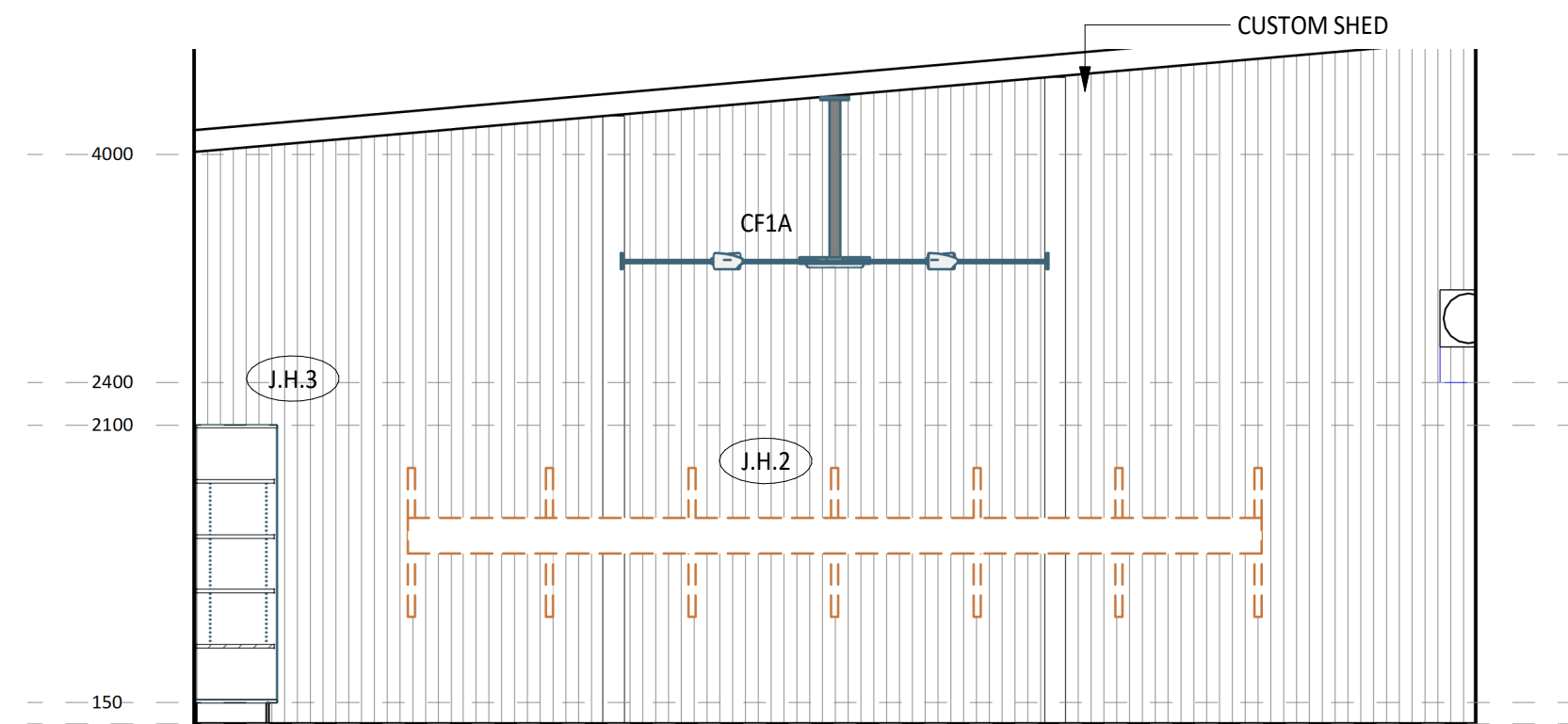
2 ELEVATION DETAIL 60-003 1 : 50
